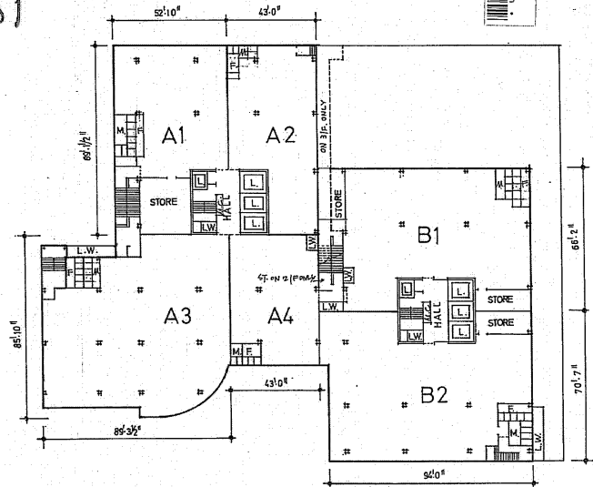
2ND. TO 3RD. FL. PLAN
