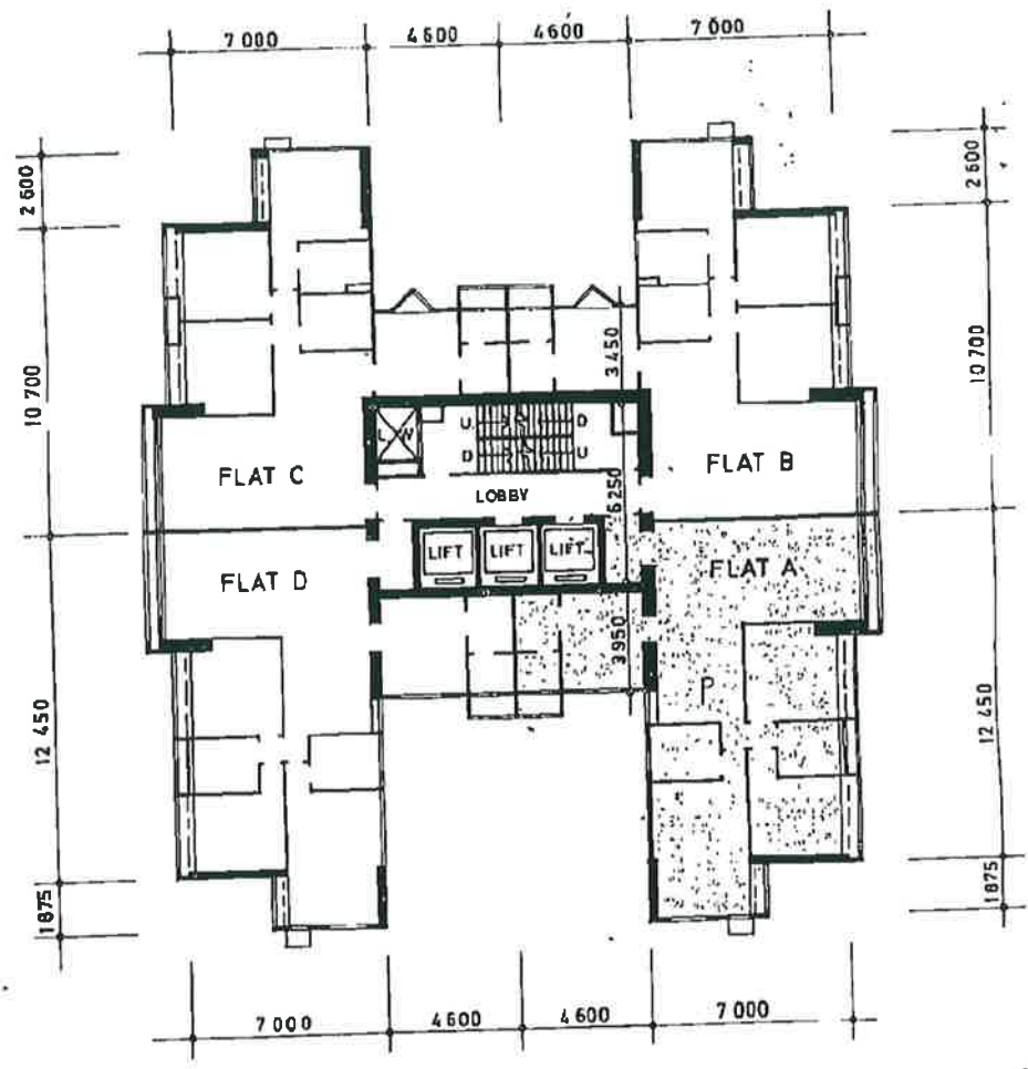
2ND-11TH FLOOR PLAN SCALE 1:250
