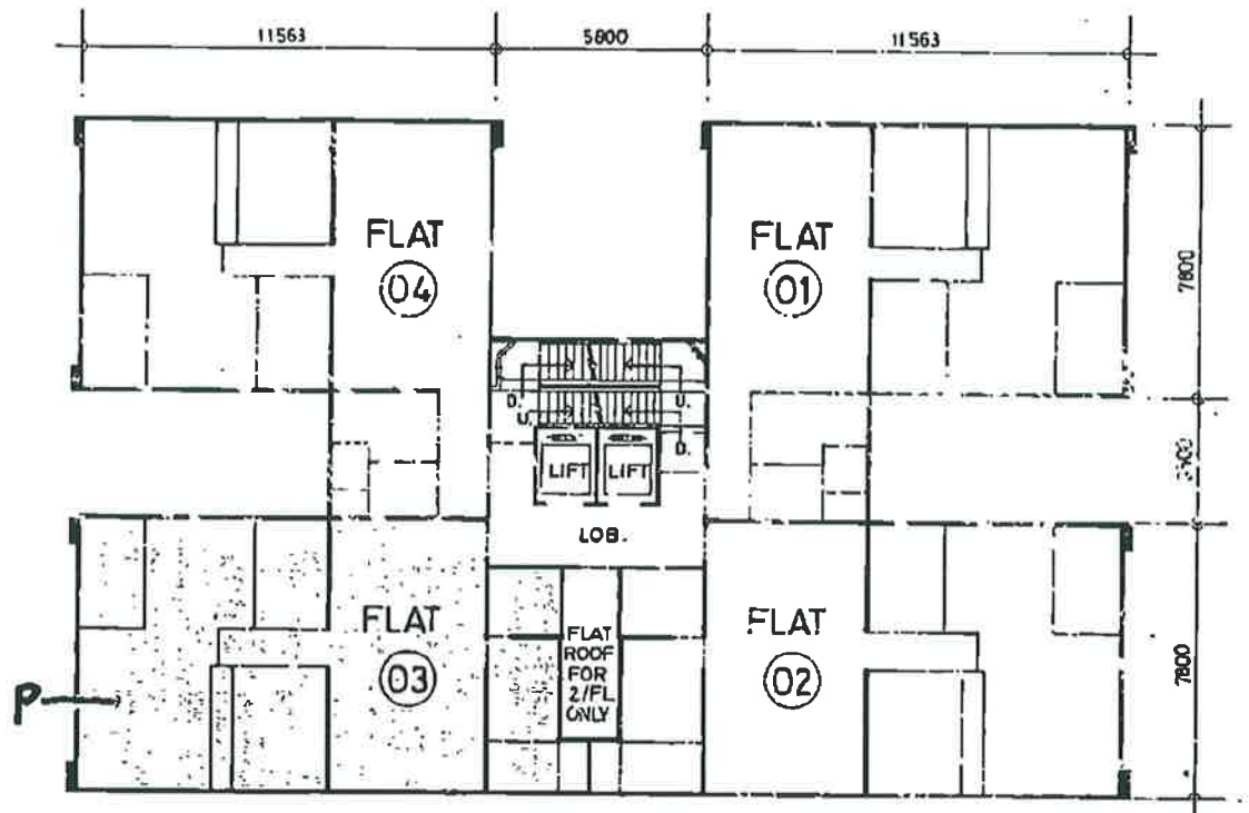
2nd TO 31st FLOOR PLAN (BLOCK 'A') SCALE 1:200
