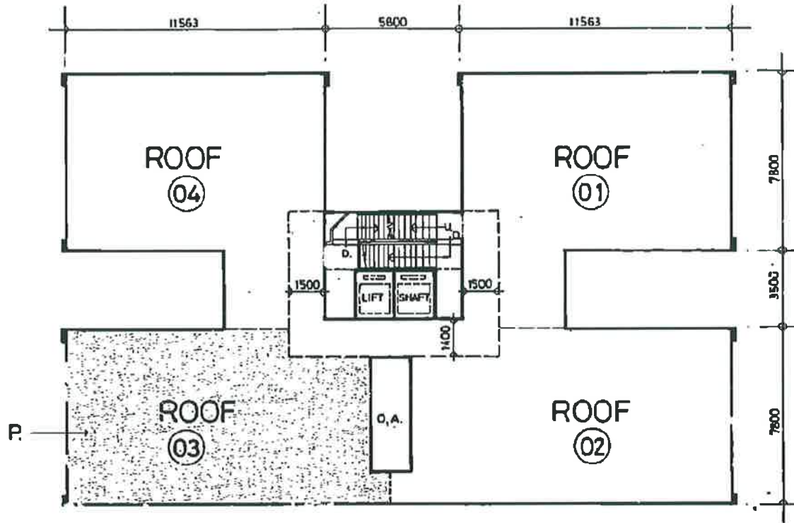
ROOF PLAN SCALE 1:200 (BLOCK 'A')
