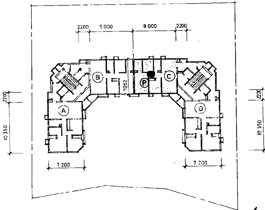
3RD - 15TH FLOOR PLAN
