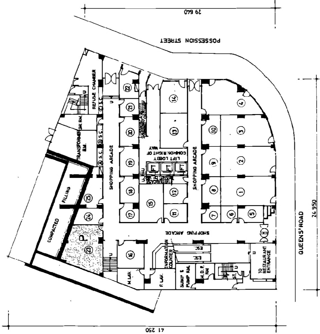
GRD. FLOOR PLAN
