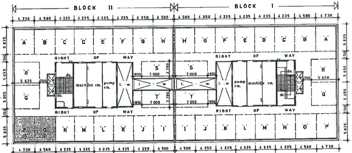
ROOF PLAN
