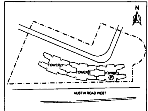
BLOCK PLAN (SITE D OF K.I.L. NO. 11080)
