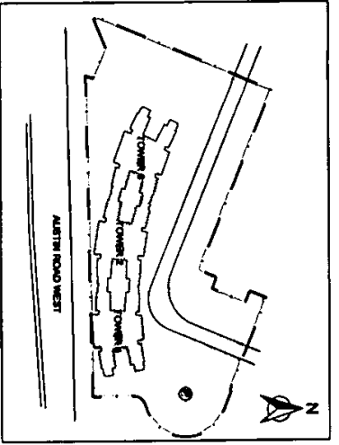
BLOCK PLAN (SITE D OF K.I.L. NO. 11080)
