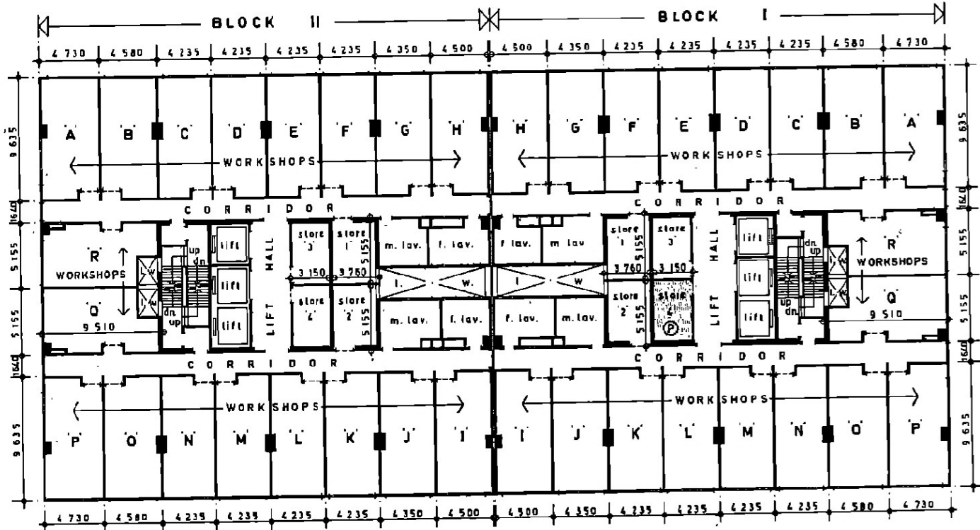
17TH FLOOR PLAN
