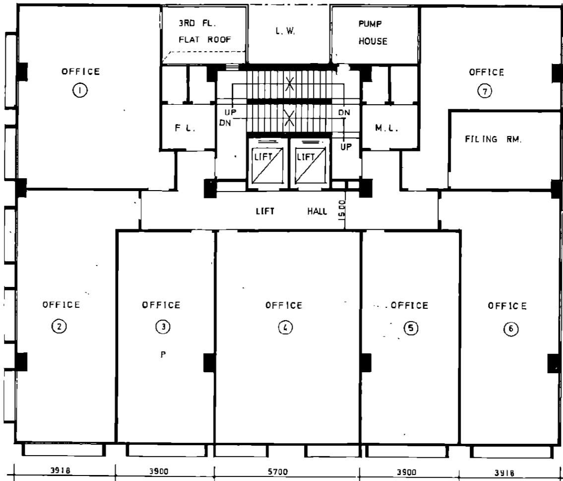
3RD & 4TH FL. PLAN
