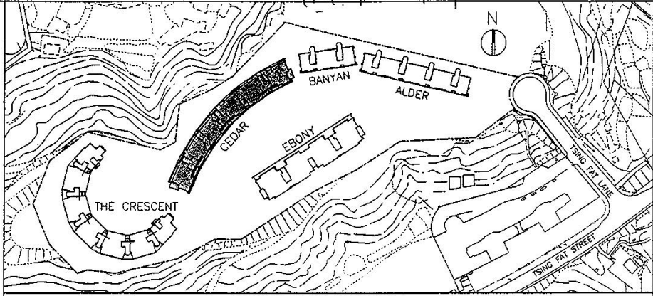
BLOCK PLAN SCALE 1 : 2500
