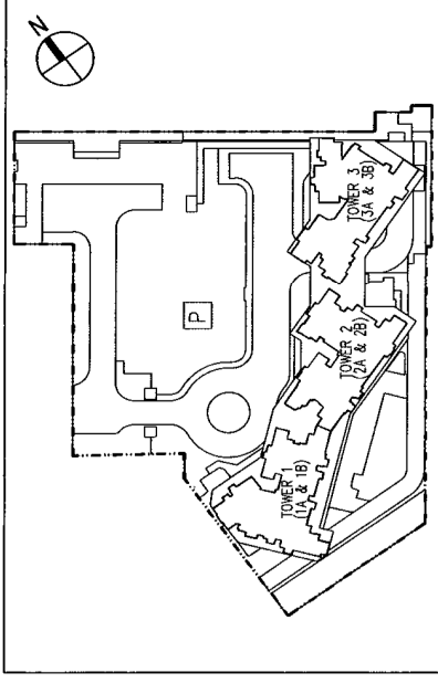
SITE PLAN (Site J of TKOTL No.70 RP) 1 : 2500
