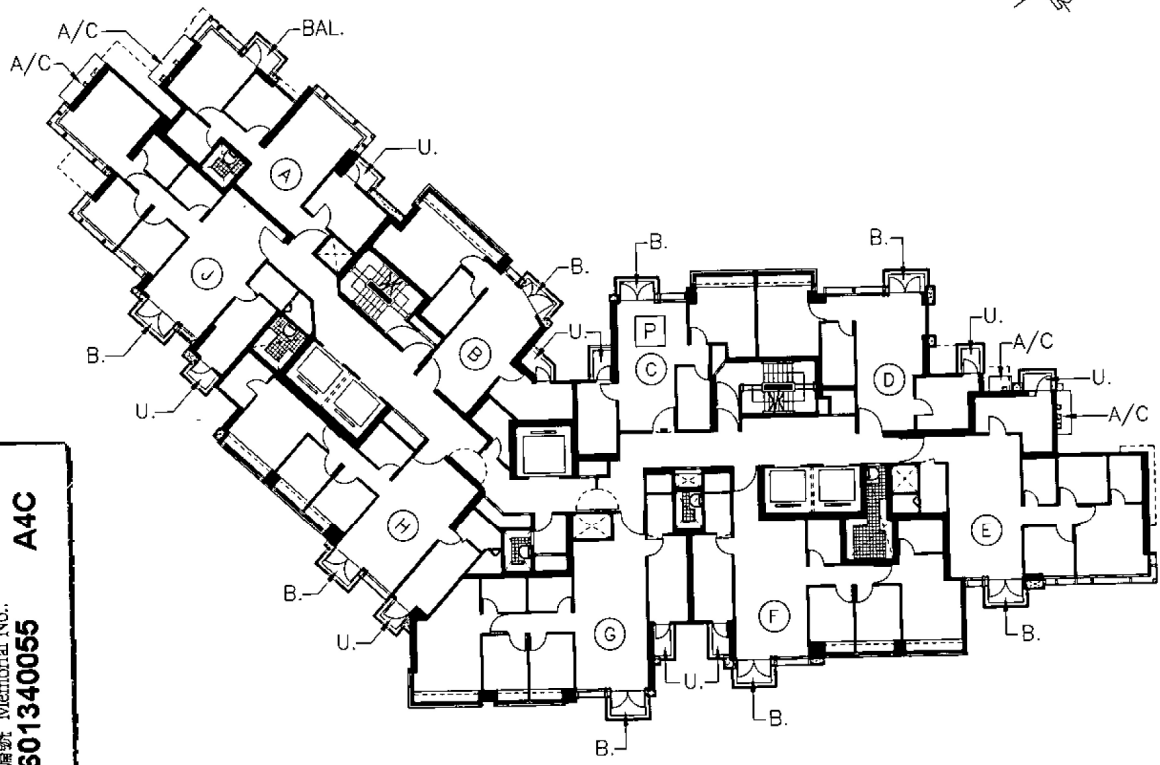
TOWER 3 - 7/F FLOOR PLAN
