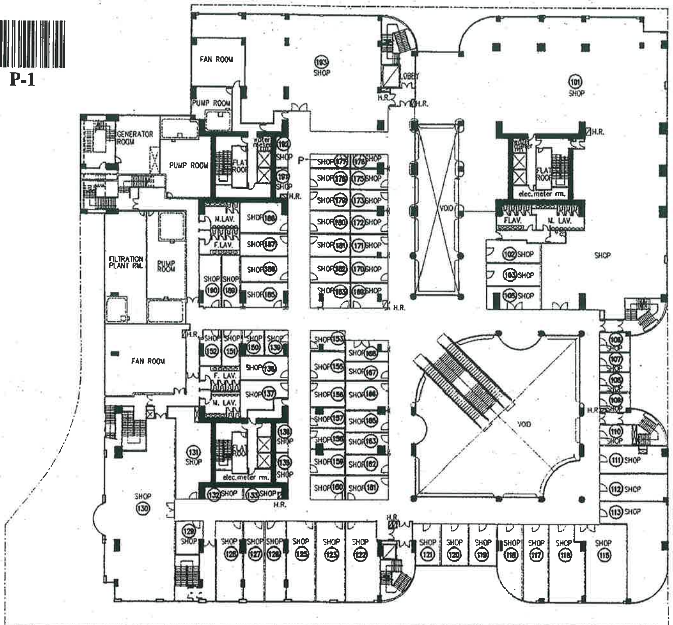
BLOCK PLAN
