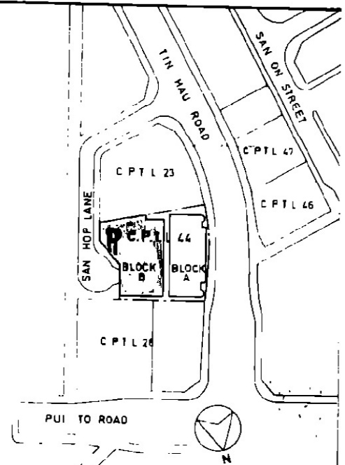
BLOCK PLAN SCALE 1 IN TO 200 FT
