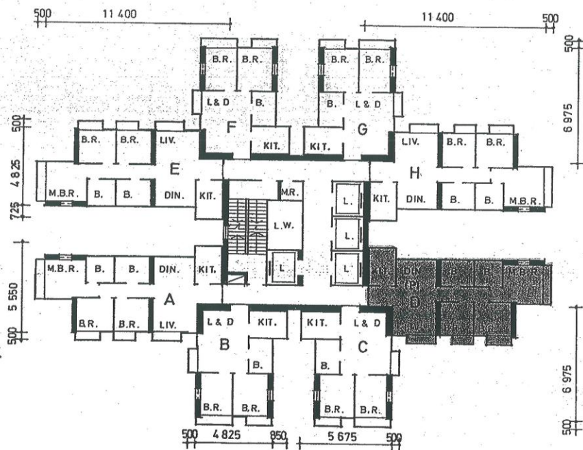
43rd FLOOR PLAN
